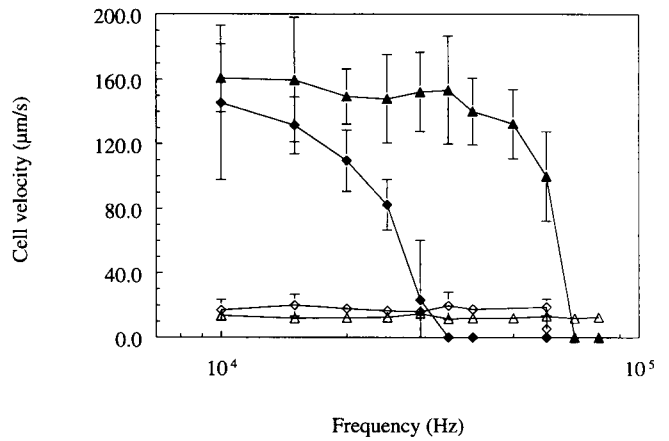
FIGURE 11 Frequency dependencies of the mean velocities for HL-60 (◆) and PBMN (▲) cells suspended in a sucrose/dextrose medium of conductivity 10 mS/m in a thin chamber containing parallel microelectrode arrays (50 \mu\text{m} width and spacing) for a flow rate of 160 \mu\text{l}/\text{min} ( \langle v \rangle = 392 \mu\text{m}/\text{s} ). The applied voltage was 0.88 V (RMS). The chamber dimensions were 375 \mu\text{m} ( H ) \times 150 mm ( L ) \times 24 mm ( W ). Each point represents the mean velocity of more than 15 cells. The open symbols correspond to the cell velocities when the electrical field was turned off.
