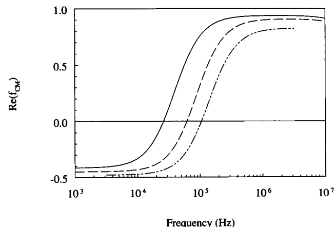
FIGURE 10 Simulated frequency dependencies of \text{Re}(f_{\text{CM}}) for HL-60 cells (---) in a suspending medium of conductivity 44 \text{ mS/m} , and HL-60 cells (—) and T-lymphocytes (— · —) in a suspending medium of conductivity 10 \text{ mS/m} . The simulations were based on the mean values of dielectric parameters for the cells determined from electrorotational measurements. For HL-60 cells, membrane capacitance = 15.6 \text{ mF/m}^2 ; membrane conductance = 220 \text{ S/m}^2 ; cell interior conductivity = 0.75 \text{ S/m} and relative permittivity = 75 ; radius = 5.8 \text{ } \mu\text{m} . For T-lymphocytes, membrane capacitance = 11 \text{ mF/m}^2 ; membrane conductance = 220 \text{ S/m}^2 ; cell interior conductivity = 0.75 \text{ S/m} and permittivity = 75 ; radius = 3.2 \text{ } \mu\text{m} .
